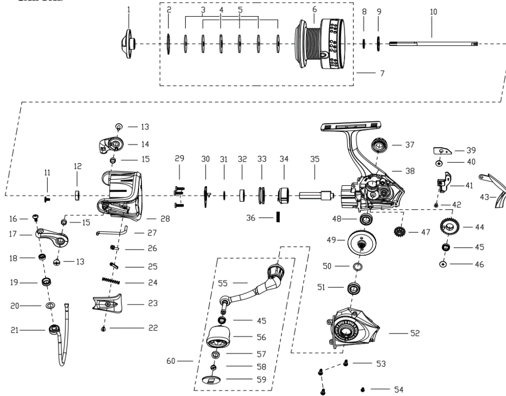
PARTS LIST OF MAXPROSP20
