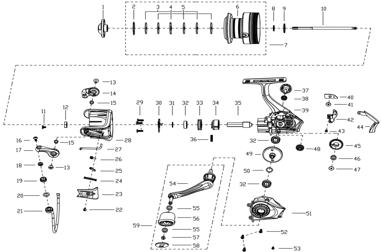
PARTS LIST OF MAXXSP30/40
